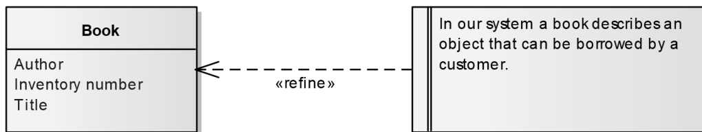
Figure 12: Class and natural language definition
