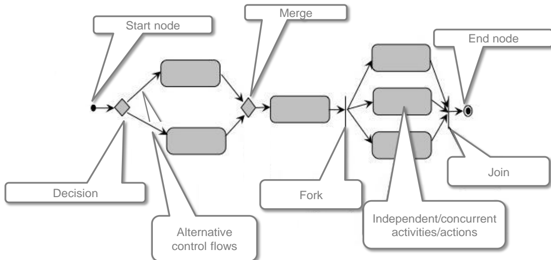
Figure 44: Using the model elements of activity diagrams
