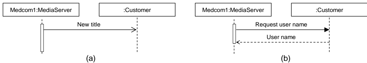
Figure 81: Modeling a) asynchronous and b) synchronous messages
