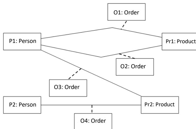
Figure 25: Example for a valid instantiation of the class diagram in Figure 24 (left hand side)
