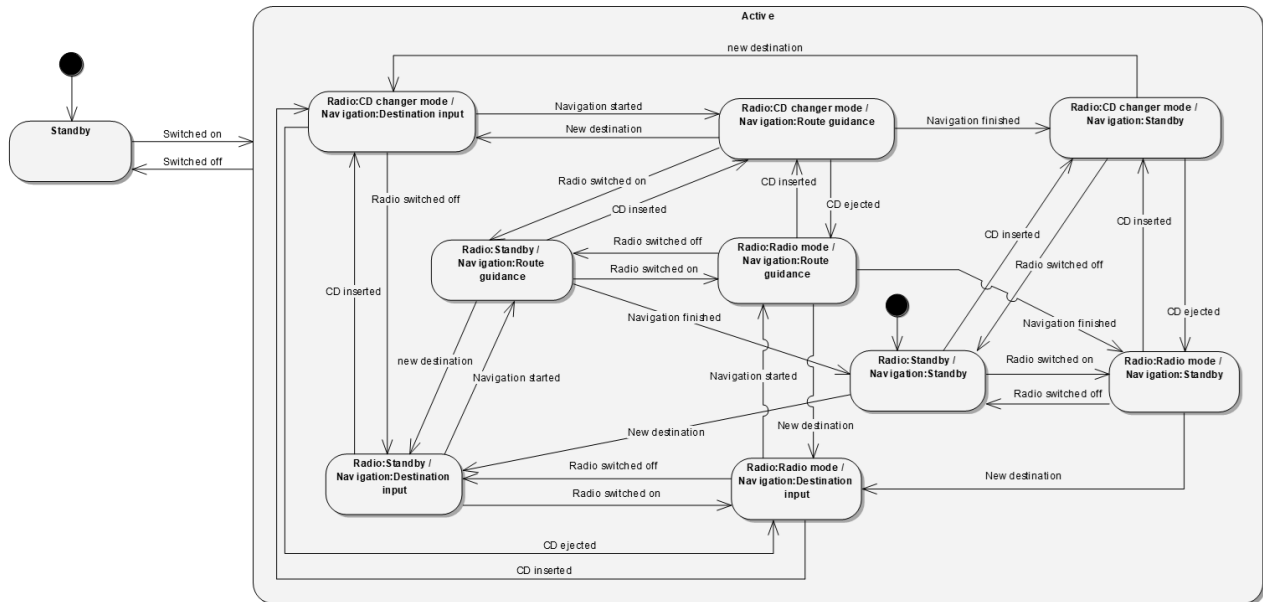
Figure 75: Resolved orthogonal regions
