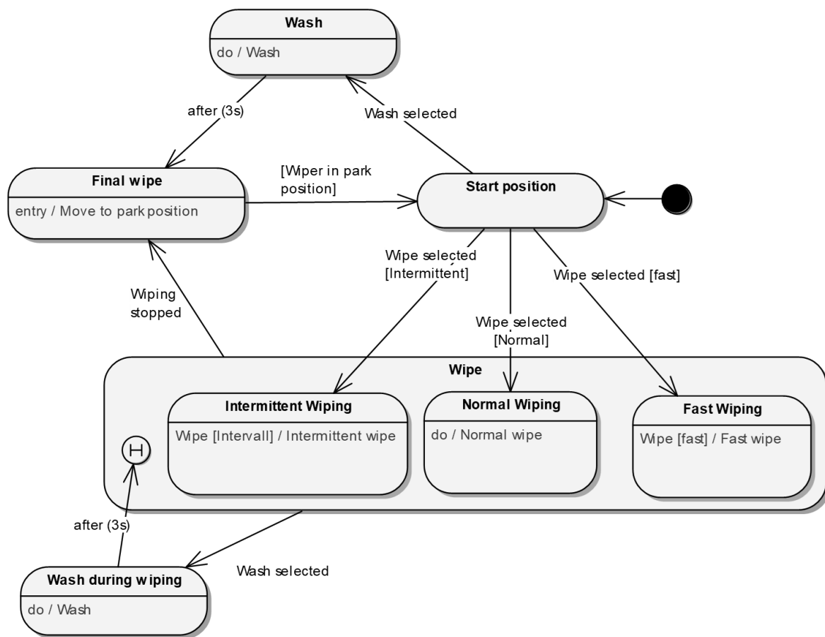
Figure 54: State diagram for a wiper system
