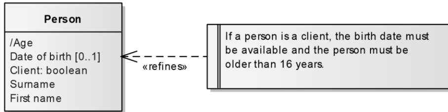
Figure 19: Modeling attribute constraints
