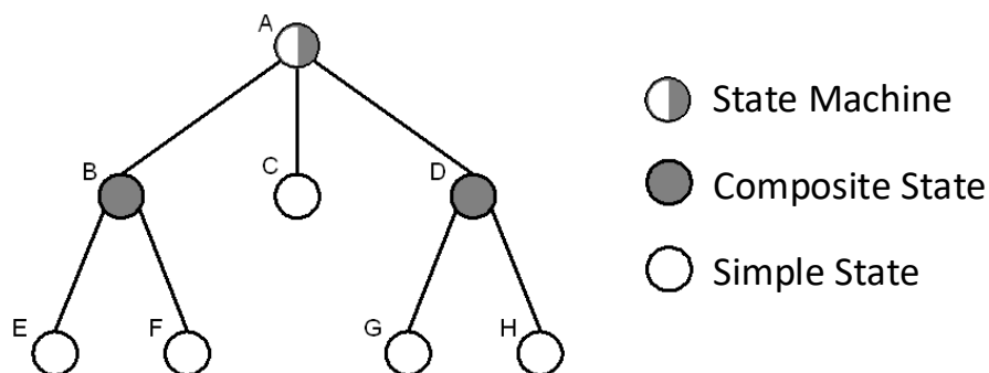
Figure 63: Hierarchical states
