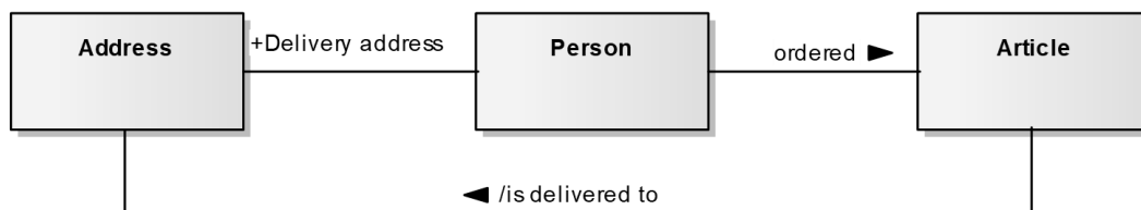
Figure 33: Derived associations
