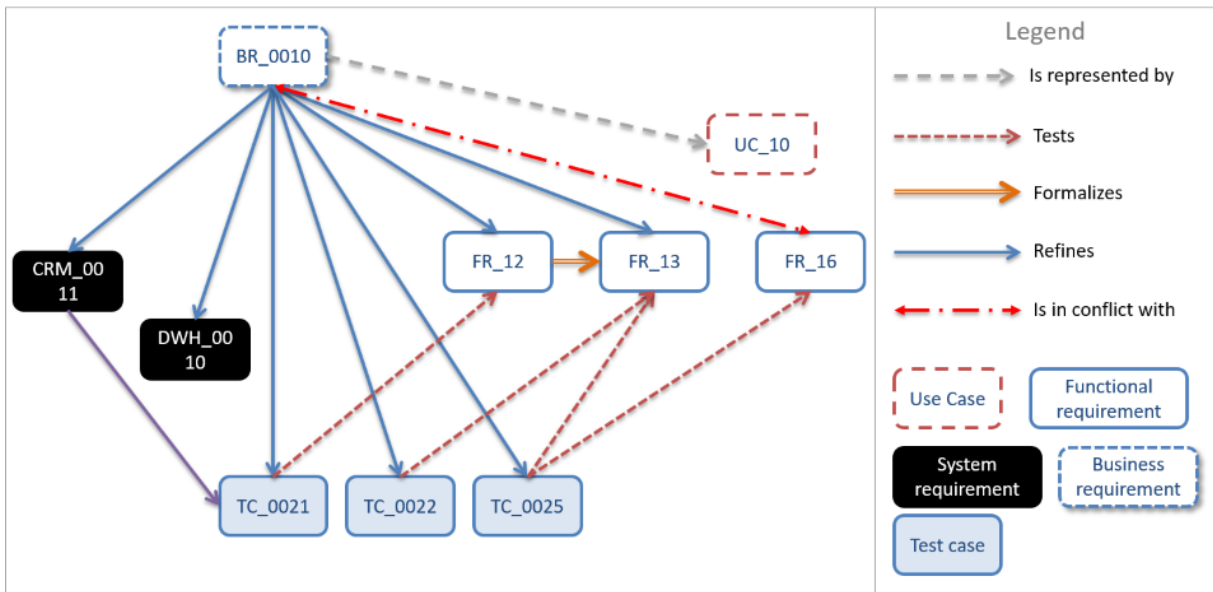
Figure 10: Traceability graph
