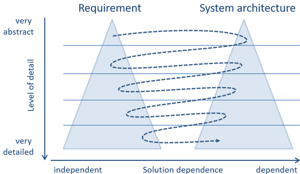
Figure 1: Twin-Peaks model
